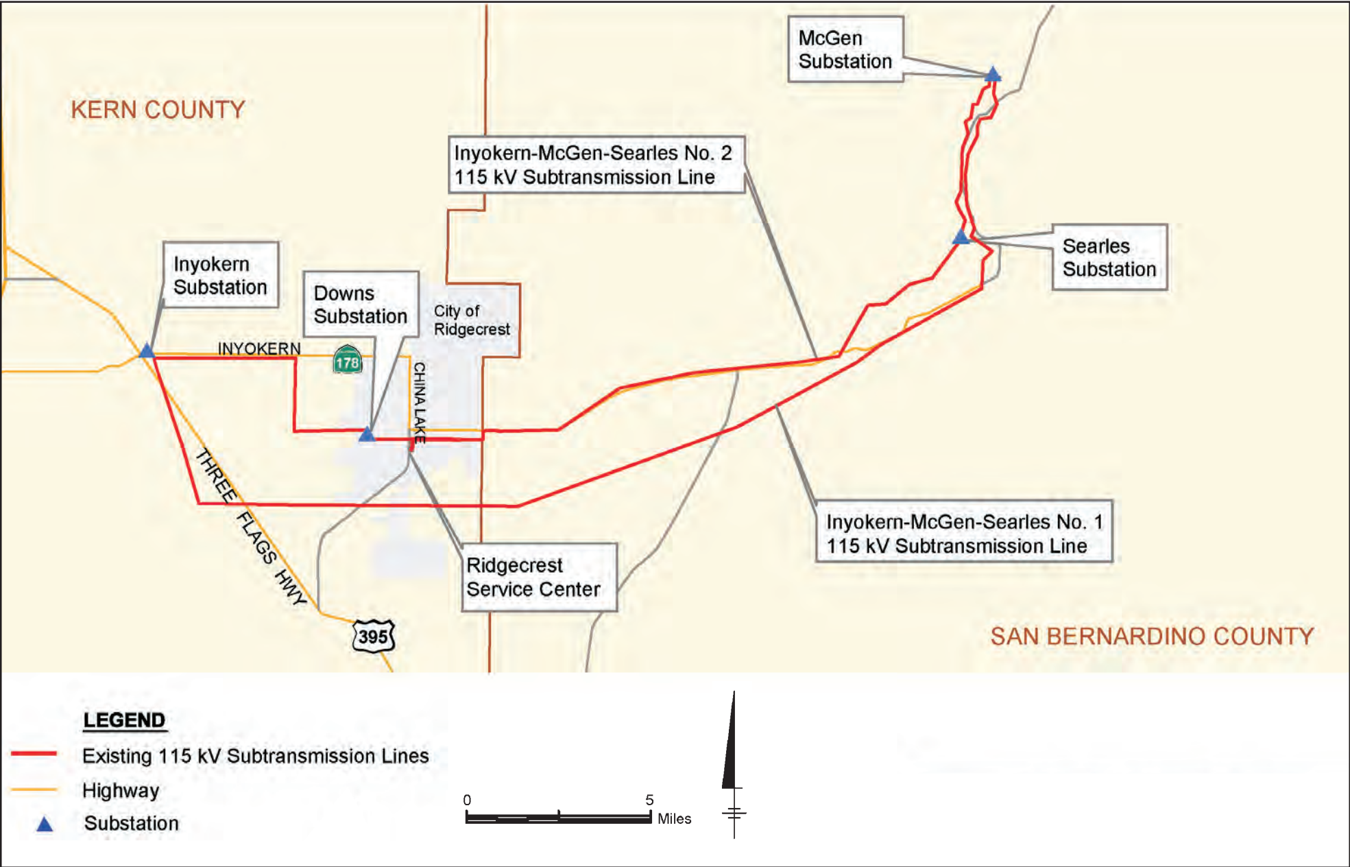
Figure B.1-8 Existing 115-kV Subtransmission Line Routes in the Vicinity of the Project Area
