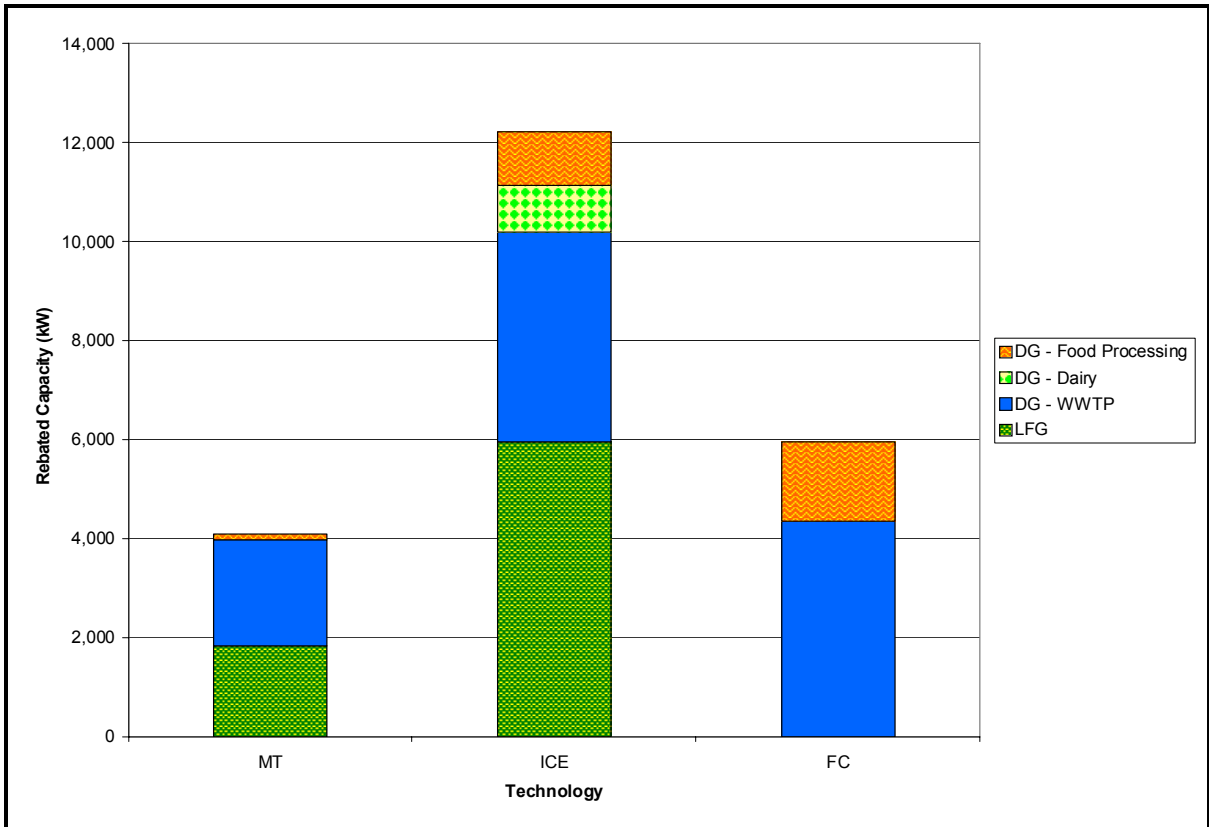
Figure 3: Contribution of Biogas Fuel Type by Prime Mover Technology
