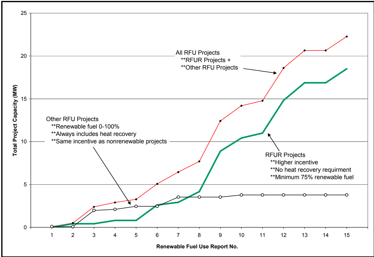
Figure 1: Project Capacity Trend (RFU Reports 1–15)
