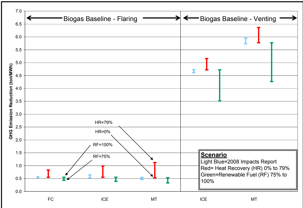
Figure 4 : GHG Emission Reduction Scenarios
