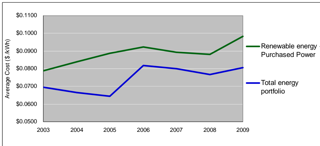
Figure 3.4 Average cost of RPS eligible sources and total energy portfolio CORRECTED
