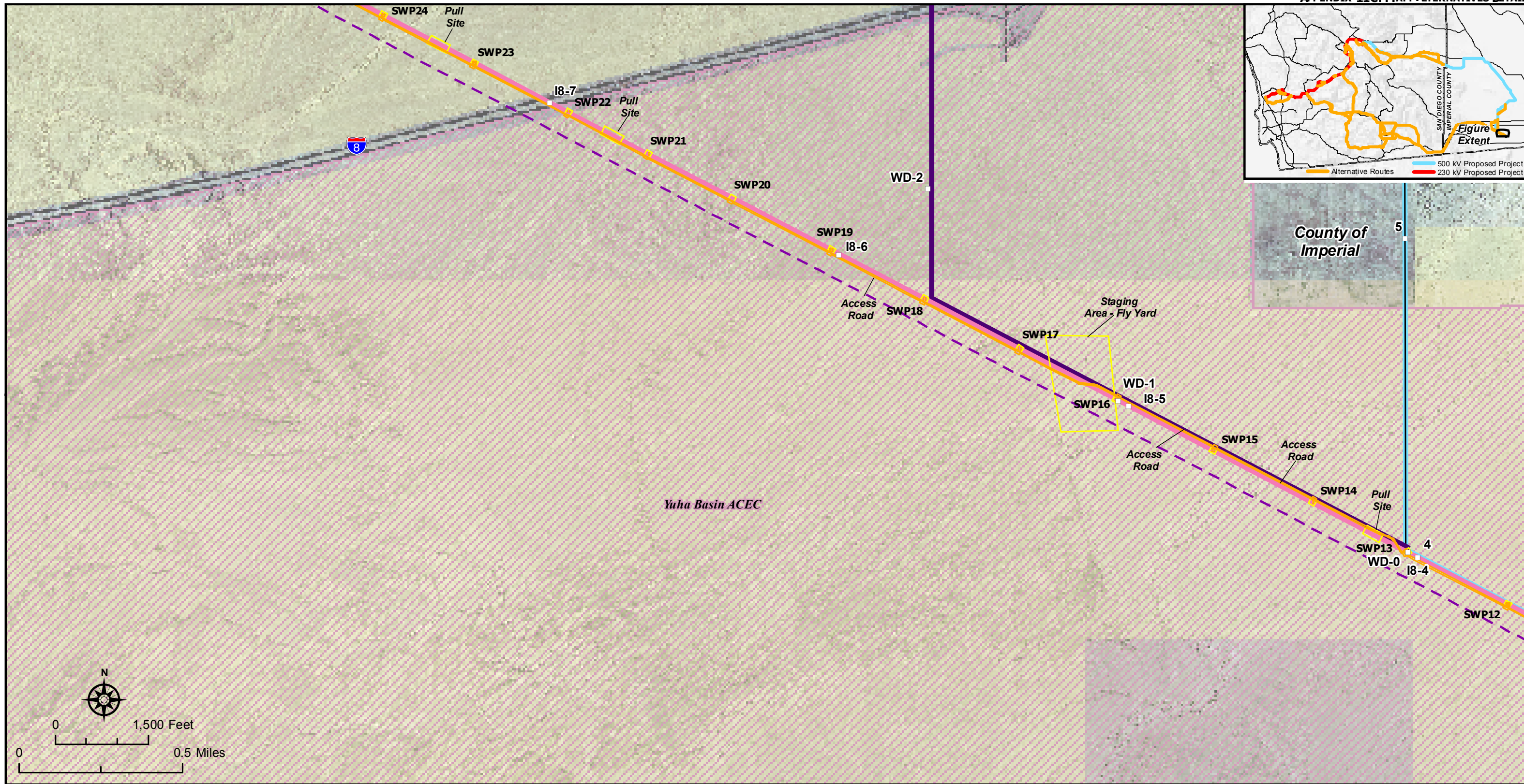
Sunrise Powerlink Project Figure Ap. 11C-36 Interstate 8 Alternative, Overhead Portion Detail
