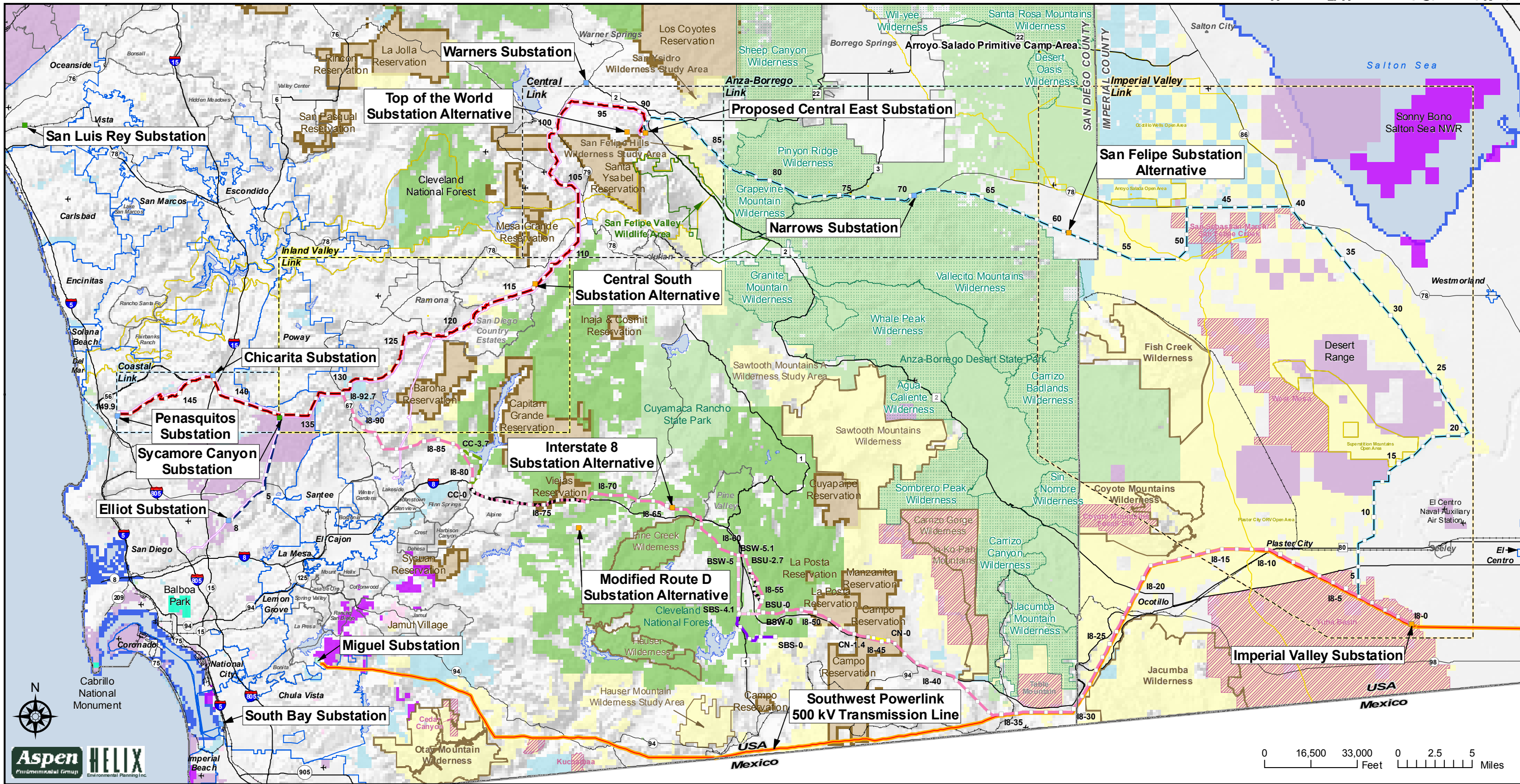
Sunrise Powerlink Project Figure Ap.1-27a Existing Southwest Powerlink Transmission Line and Interstate 8 Alternative
