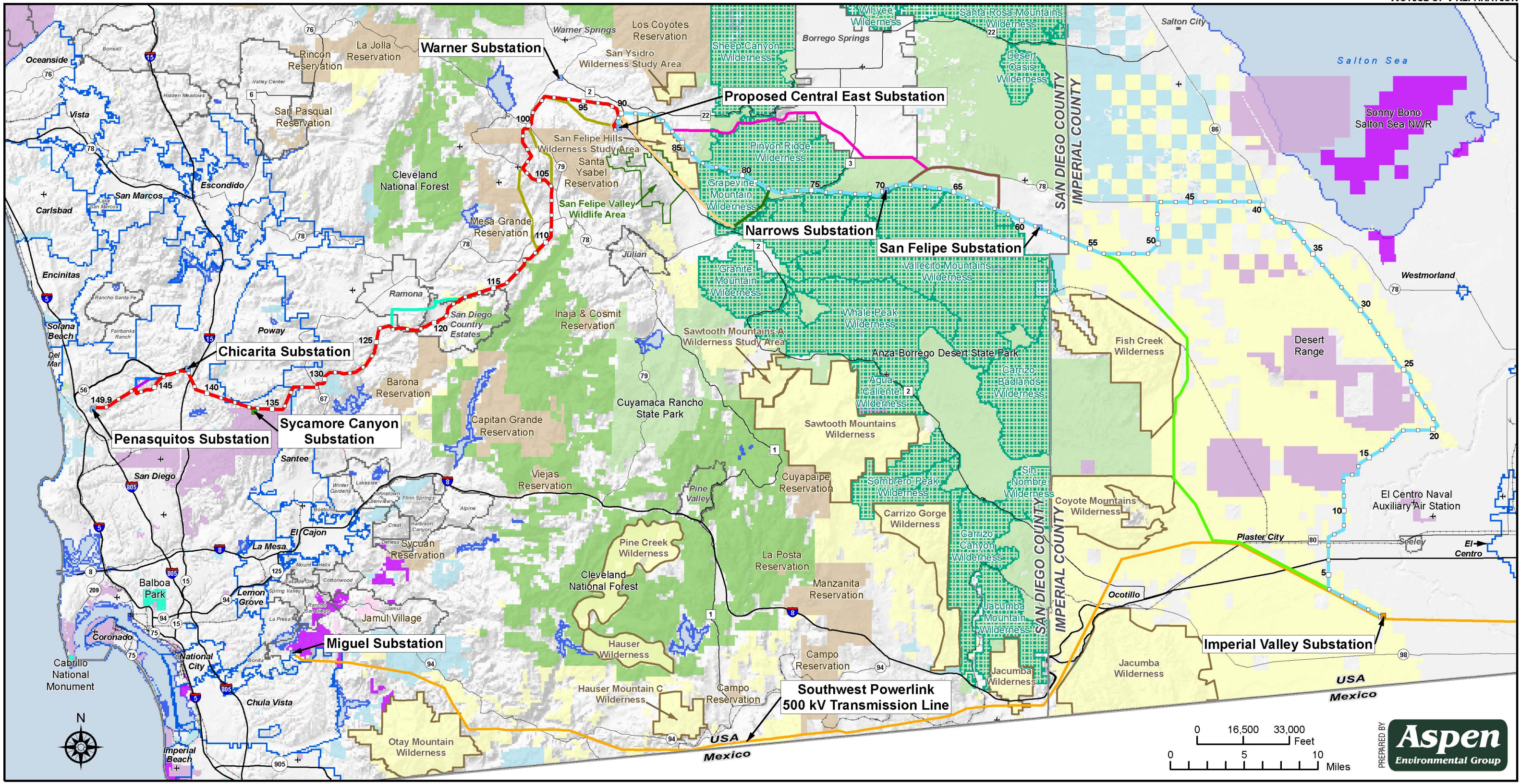
Sunrise Powerlink Project Figure 7 SDG&E Alternatives Fully Evaluated and Carried Forward
