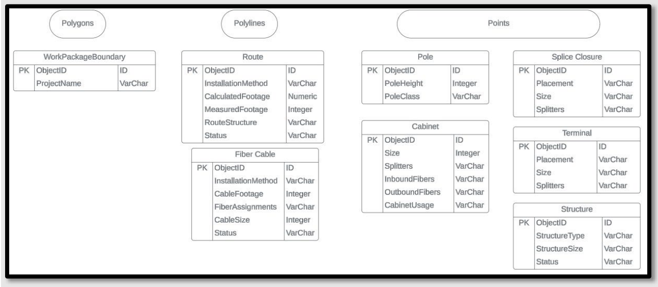
Figure 1. Data Schema for HLD
