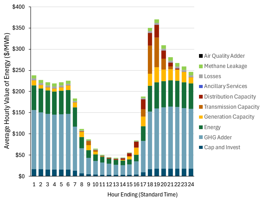
Figure 10-5. Average Hourly Avoided Costs (PG&E Climate Zone 12, 20-year levelized value of 2026 resource) - 2026 ACC
