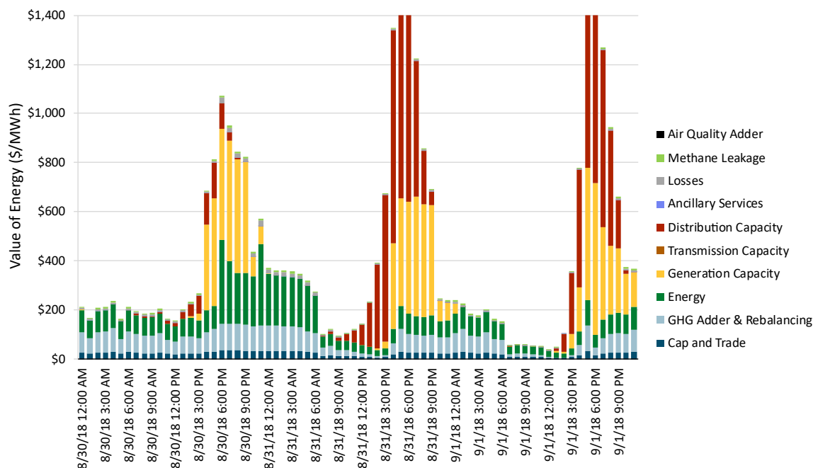
Figure 10-7. Hourly Avoided Costs for Three Days Beginning August 30th (PG&E Climate Zone 12, 20-year levelized value of 2026 resource)* - 2026 ACC
