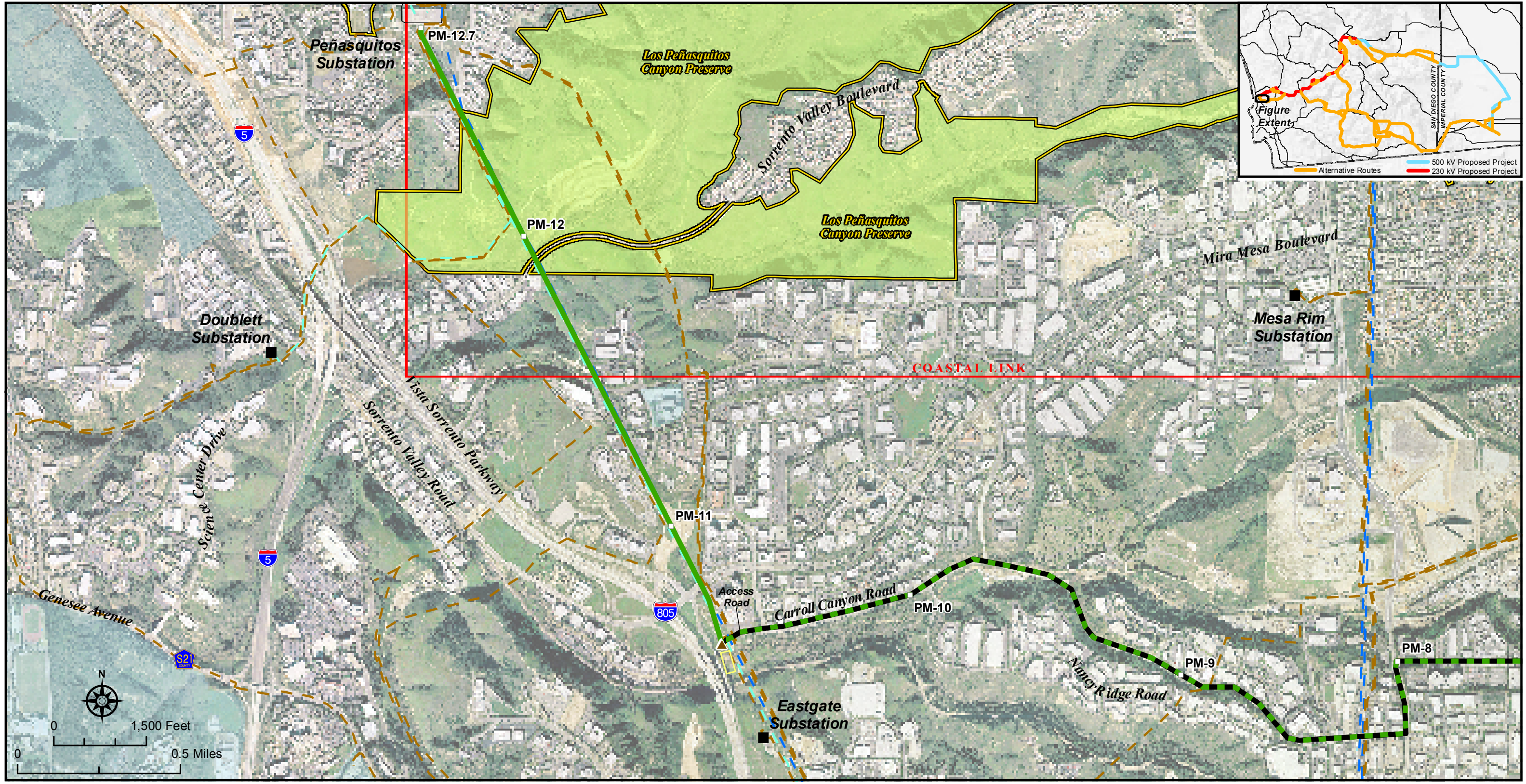
Sunrise Powerlink Project Figure Ap. 11C-31 Pomerado Road to Miramar Area North Alternative Detail
