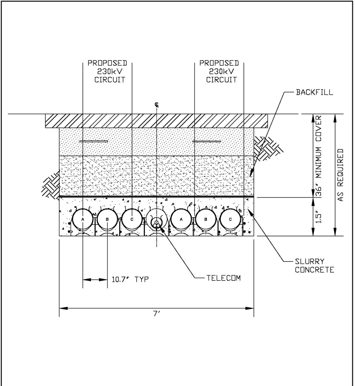
Figure B-26 Typical 230 kV Duct Bank: Coastal Link (horizontal configuration)
