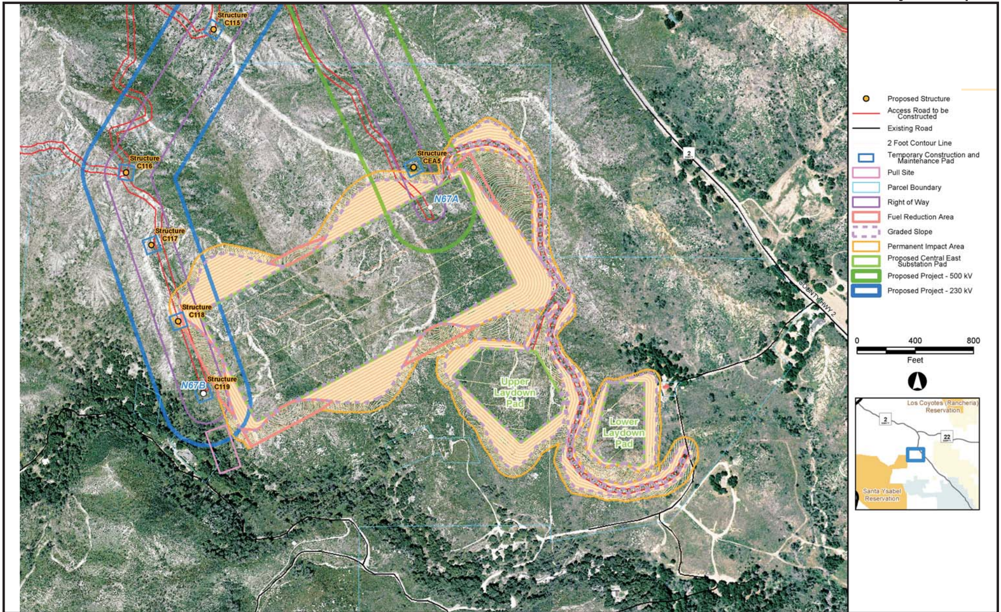
Figure B-36 Central East Substation: Grading Plan
