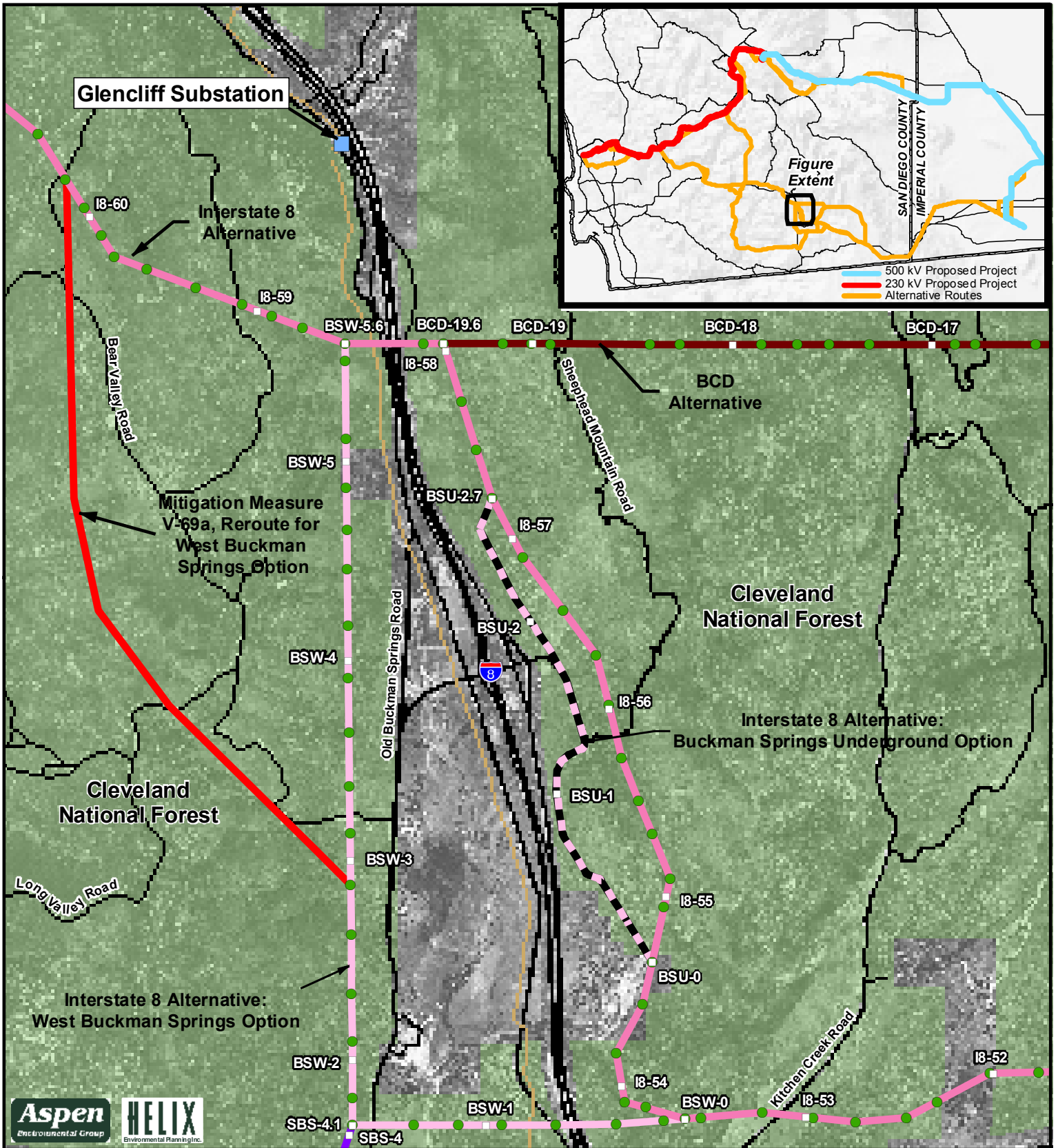
Sunrise Powerlink Project Figure E.1.3-14C Buckman Springs Alternative Reroute per Mitigation Measure V-69a
