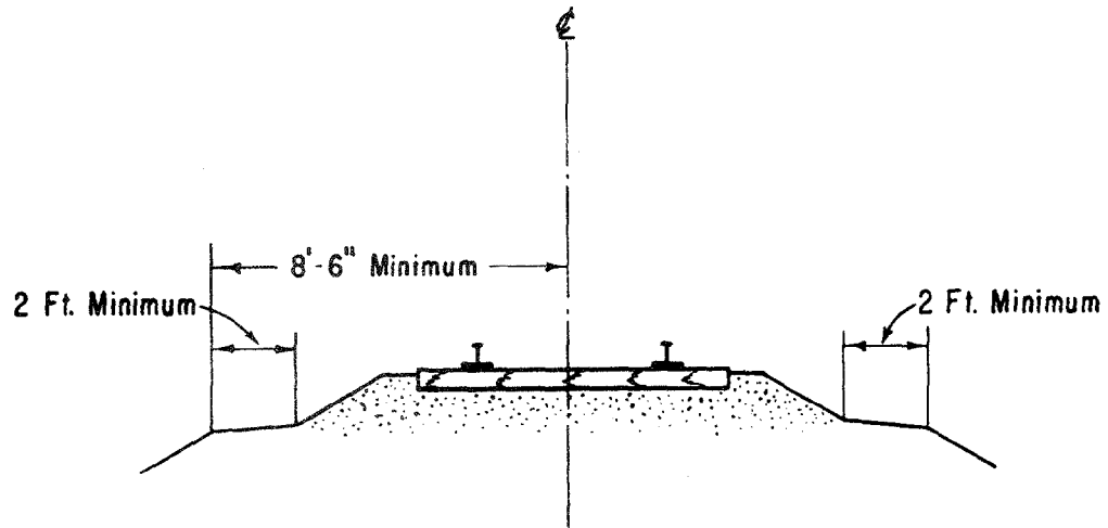
STANDARD No. 1 WALKWAYS ALONG MAIN LINE TRACKS
