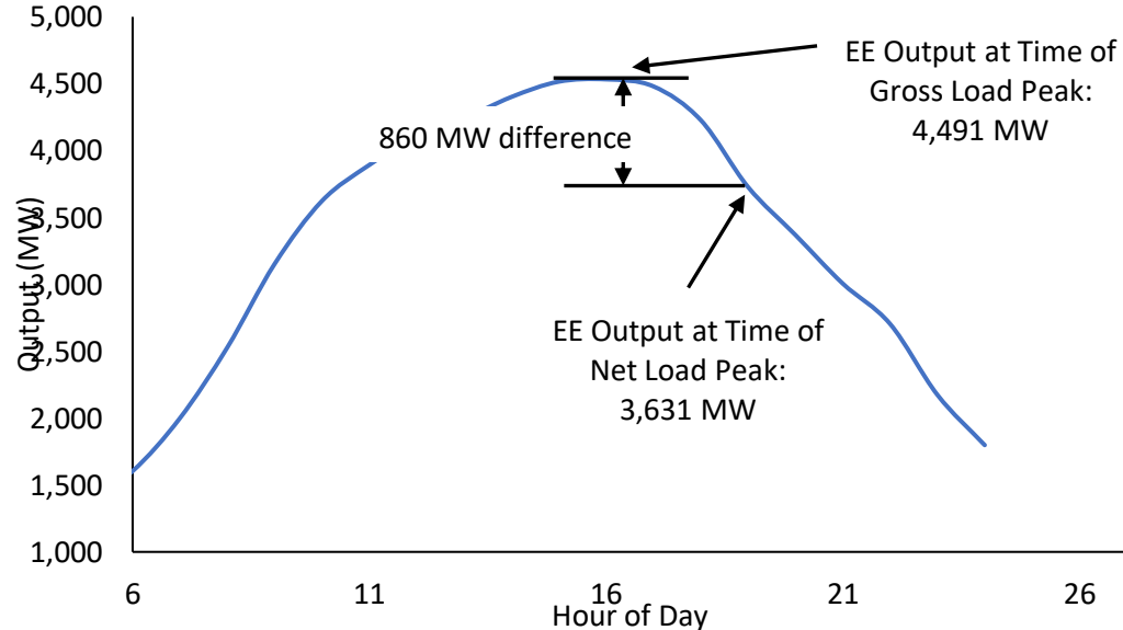
Figure 4.2 Energy Efficiency Output at Time of Gross and Net Load Peaks
